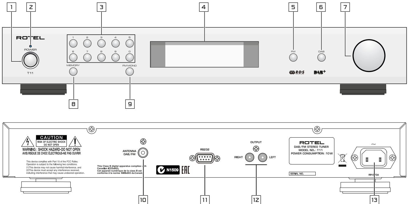
Figure 1: Controls and Connections Commandes et Branchements Bedienelemente und Anschlüsse Controlles y Conexiones
